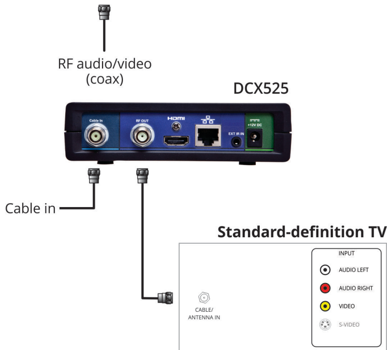
Figure 4: Connecting an SDTV — Single Connection for Video/Audio
